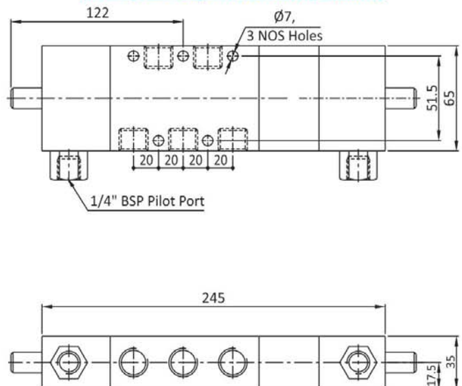
Size : 1/2" BSP (Dimensions are in mm)
